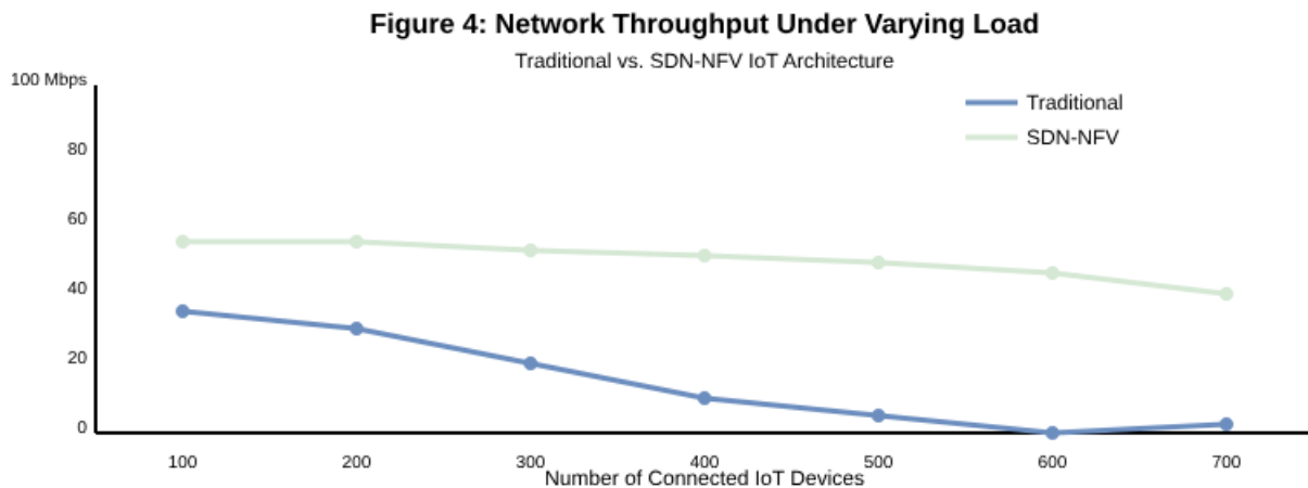
Figure 4: Network Throughput Under Varying Load
