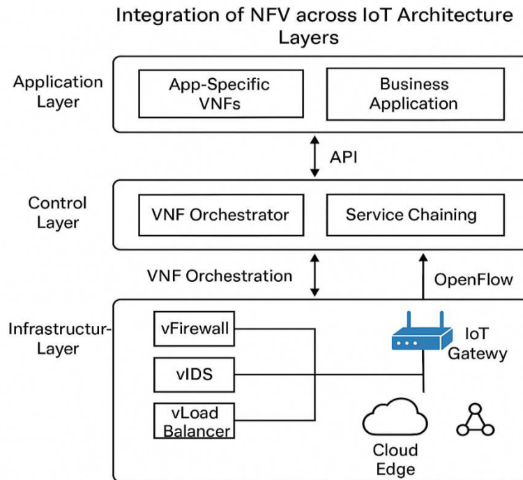
Figure 2: Integration of NFV across the Application, Control, and Infrastructure layers of the proposed SDN-based IoT architecture.
